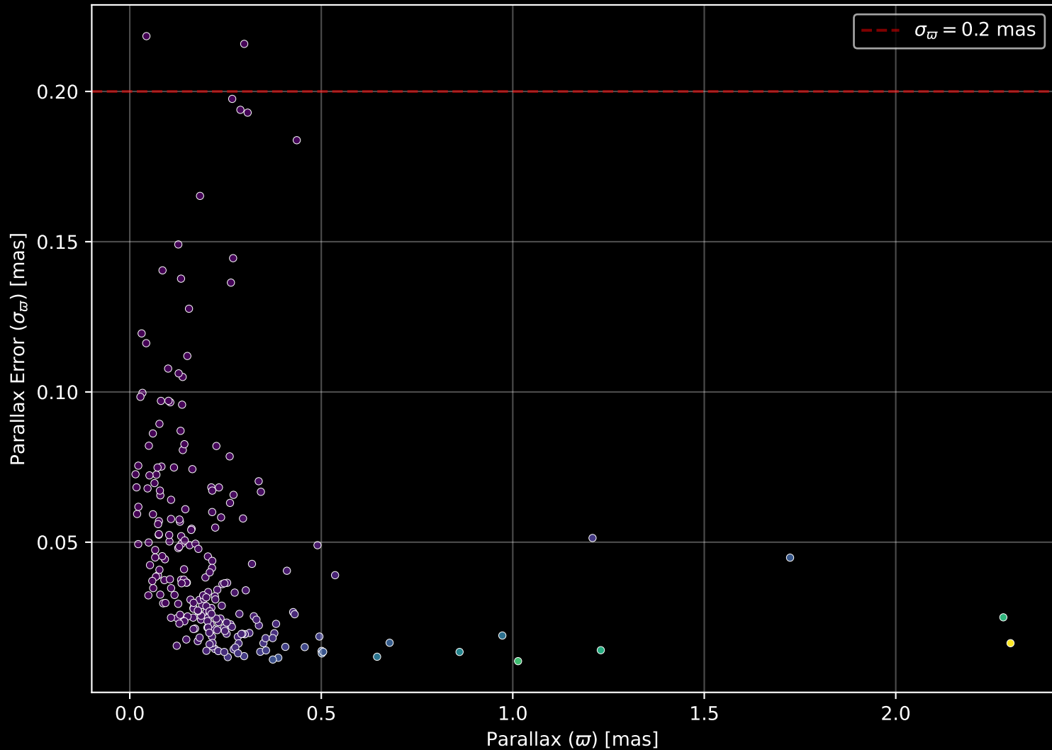
APOGEE DR17 Field: [296+00] Parallax Quality (n= 227)
