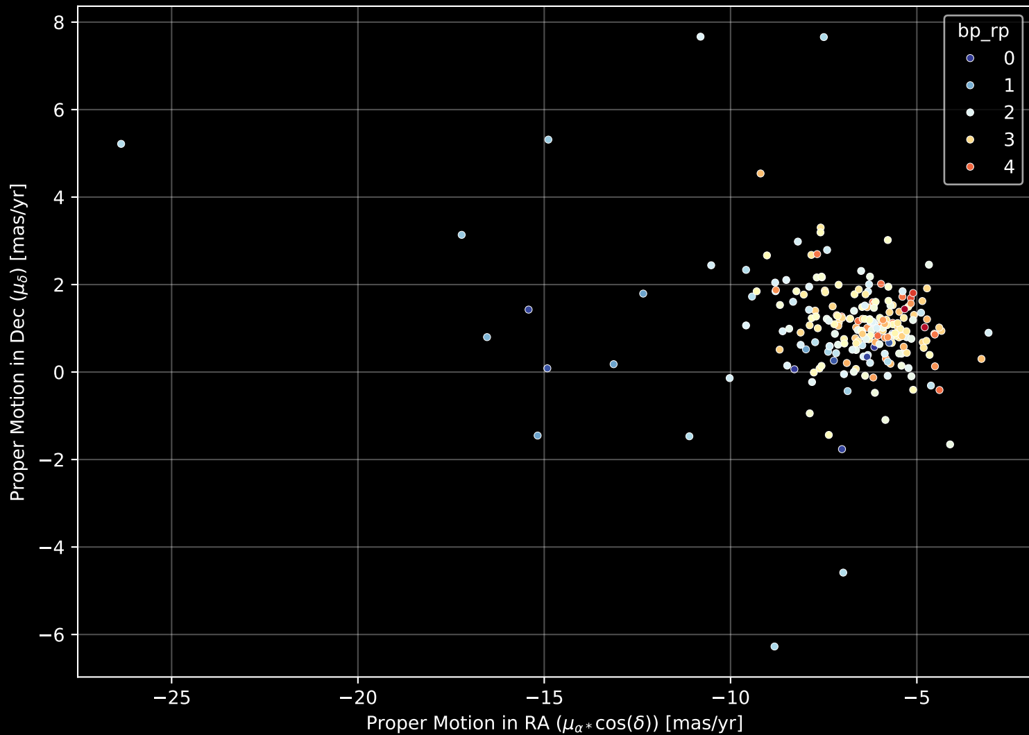
APOGEE DR17 Field: [296+00] Proper Motion Diagram (n= 227)
